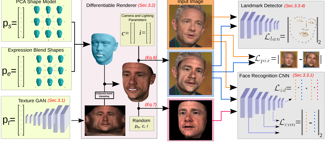
Figure 2: Detailed overview of the proposed approach. A 3D face reconstruction is rendered by a differentiable renderer (shown in purple). Cost functions are mainly formulated by means of identity features on a pretrained face recognition network (shown in gray) and they are optimized by flowing the error all the way back to the latent parameters ( p_s, p_e, p_t, c, i , shown in green) with gradient descent optimization. End-to-end differentiable architecture enables us to use computationally cheap and reliable first order derivatives for optimization thus making it possible to employ deep networks as a generator (i.e., statistical model) or as a cost function.
