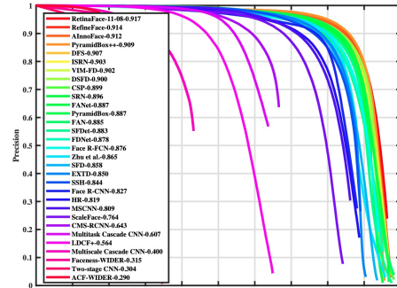
Figure 7. Precision-recall curves of RetinaFace (ResNet-152) on the WIDER FACE test Hard subsets.
