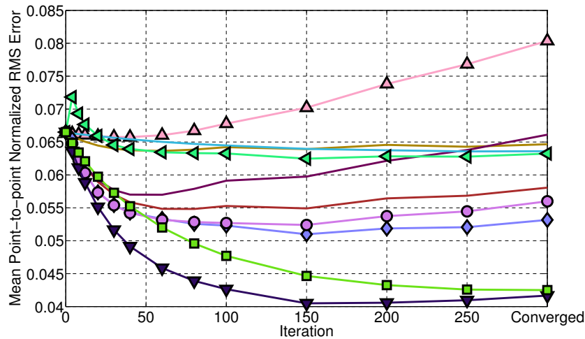
(b) Project-Out IC
