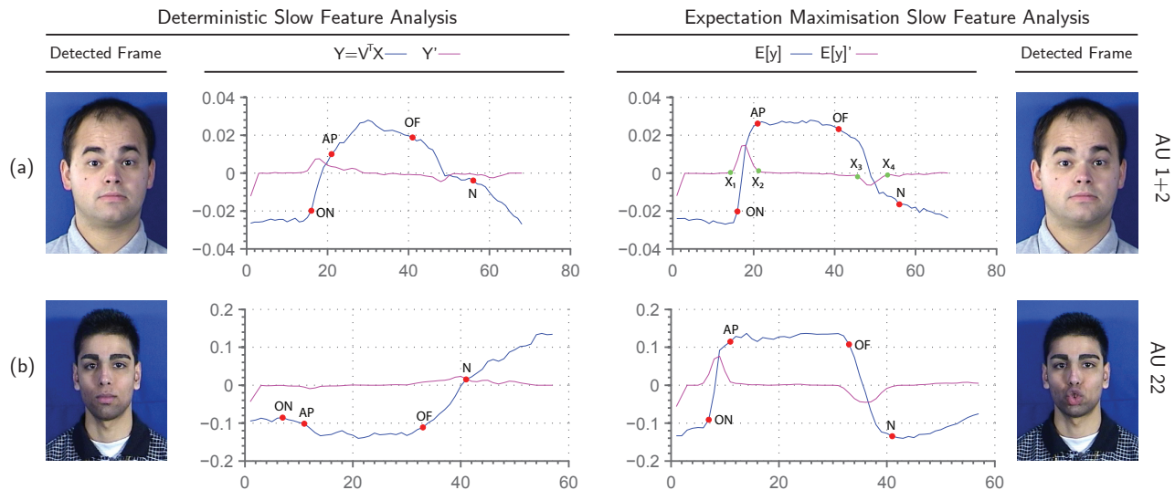
Figure 3: Comparing the derived latent space (i.e. slowest varying feature) for SFA and EM-SFA, obtained when applying the algorithms on two different videos. The space ( E[y] ) along with the gradient ( E[y]' ) is shown. The true points where the AU temporal phase changes are shown with red markers. (ON - change from neutral to onset, AP - change from onset to apex, OF - change from apex to offset, N - change from offset to neutral).
