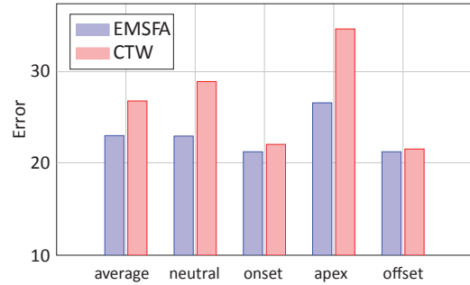
Figure 4: Results obtained when comparing EM-SFA with DTW to CTW, for all temporal phases of AUs.
