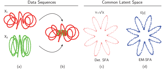
Figure 2: Application of deterministic SFA and EM-SFA on two synthetic data sequences \mathbf{X}_1, \mathbf{X}_2 (a,b). The resulting common latent space is shown in (c),(d).
